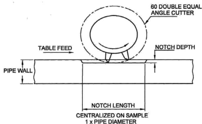
FIG. 8 NOTCH METHOD
