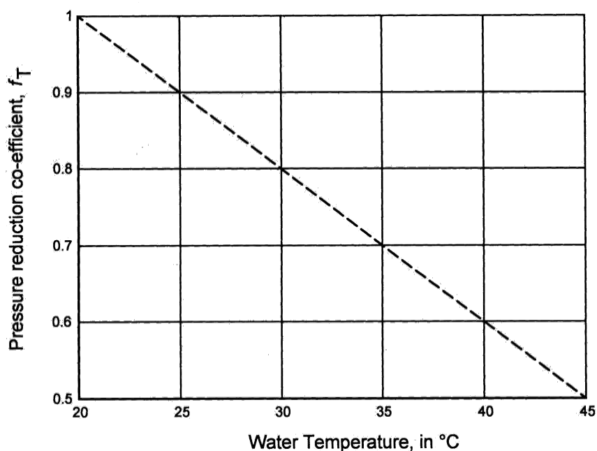
FIG. 1 PRESSURE REDUCTION CO-EFFICIENT FOR WATER TEMPERATURES ABOVE 20°C
