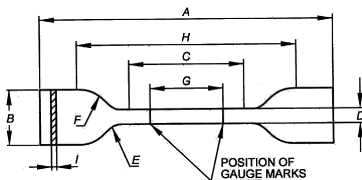
FIG. 5 TYPE 2 TEST PIECE
